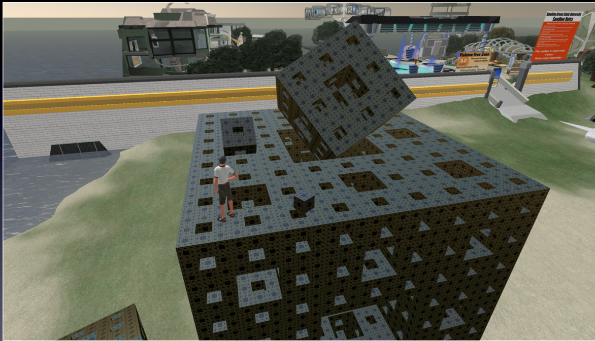
Menger Sponge: 4 geometric iterations, 3 textured iterations
