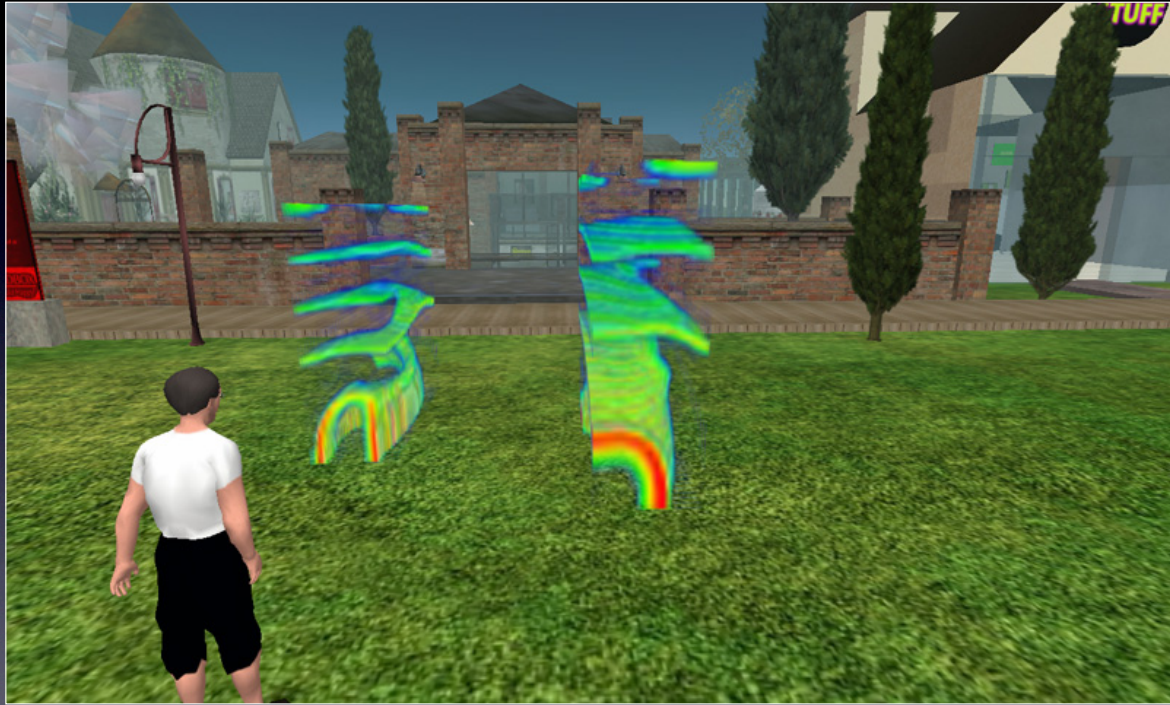
Volume visualisation of helix wave formation in fluid flow
