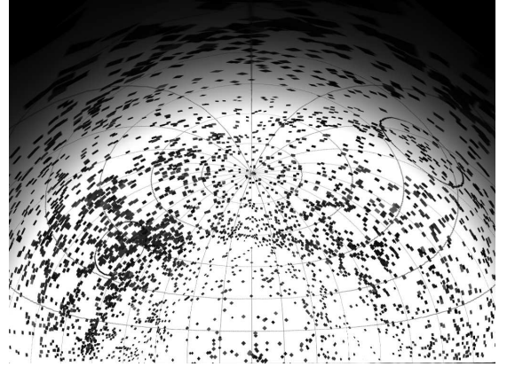
Figure 5: Projection of southern HICAT galaxies in the velocity range 0\text{--}10000\text{ km s}^{-1} suitable for display on a Swinburne MirrorDome. Note the extensive (but correct) distortion towards the top and sides of the image where glancing projections off the mirror occur, and the deliberate dimming of the image to maintain uniform brightness over the dome.
