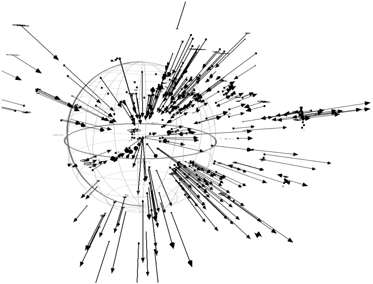
Figure 9: Three-dimensional comparison of galaxy distance measures for the LVHIS sample. See text for further information.
