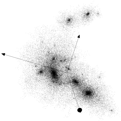
Figure 7: Zoomed view of a section of the halo distribution of the previous figure. Real-time rotation of the visualization, and/or stereoscopic display of same, conveys substantially more information than this figure can hope to.
