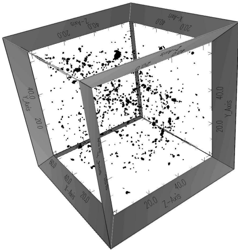
Figure 6: Overall view of halo distribution in a \Lambda WDM simulation in a 64 h^{-1} Mpc box.
