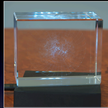
Density too low: 6df galaxy survey data
