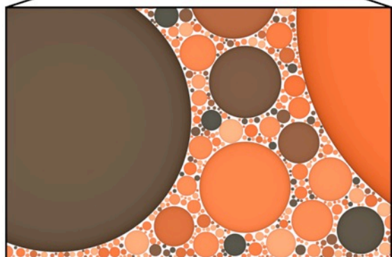
Fig 7. Illustration of self similarity across scales.
