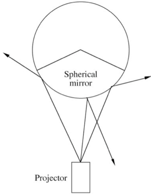
Figure 3. Scattering of light from a data projector through a wide angle by reflecting it off a spherical mirror surface. The mirror is typically located near the rim of the hemispherical dome.
